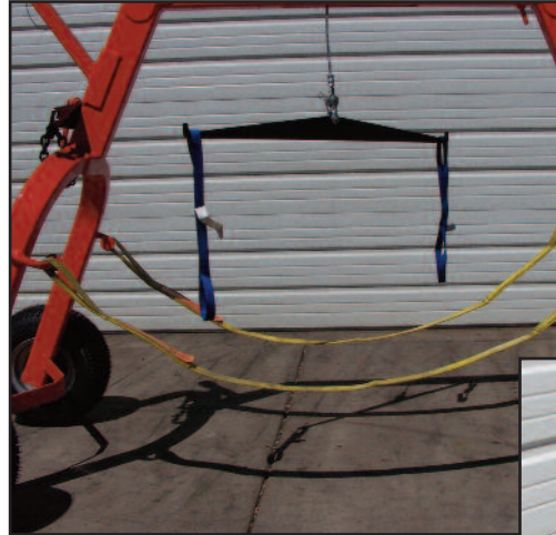
Spreader Bar Attached To Winch Line Lifting & Main Load Straps
